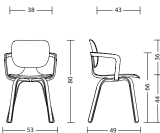
com66 with arm supports: 6 kg without arm supports: 5 kg
