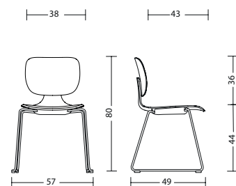
com55o without arm supports: 6 kg
