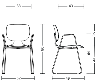
com55 with arm supports: 7 kg without arm supports: 6 kg
