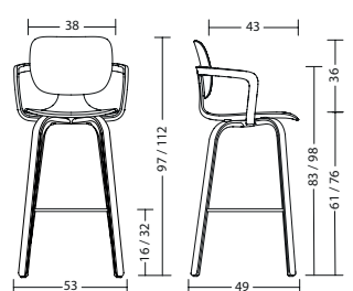
com66h with arm supports: 8 kg without arm supports: 7 kg
