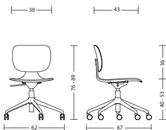
com77 without arm supports: 8 kg
